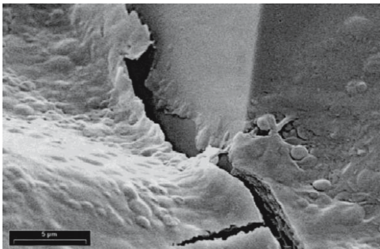
Figure 2. Scanning electron (SEM) micrograph of Beacon Sandstone, McMurdo Dry Valley (Antarctica), showing cells of Chroococcidiopsis embedded in an exopolysaccharide matrix on quartzite crystal. (Image reprinted with permission from Banerjee et al., 2000.)
