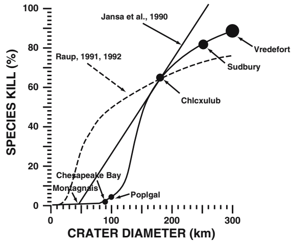
Figure 1. Poag's (1997) modifications of the Raup (1991) "kill curve" showing that only impacts producing craters much greater than 100 km in diameter are capable of producing mass extinction. (From Poag, 1997.)
