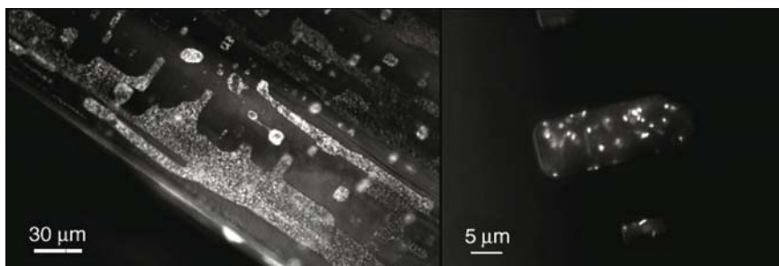
Figure 3. Localisation of pre-stained haloarchaea in fluid inclusions of artificial halite. Cells were stained with the LIVE/DEAD BacLight kit prior to embedding. Low (left panel) and high (right panel) magnification of Halobacterium salinarum NRC-1 cells. Cells were observed with a Zeiss Axioskope fluorescence microscope.
