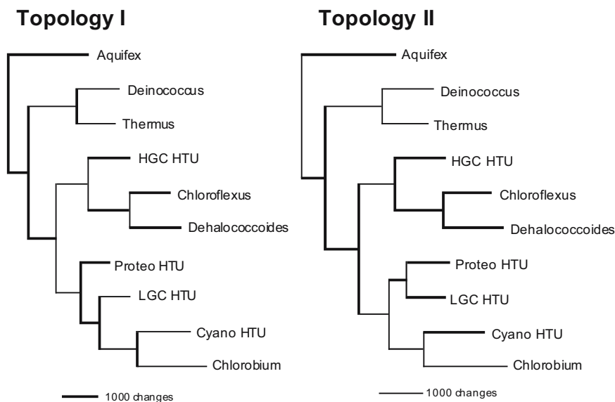
Figure 4. Trees generated by HTU analyses using MP showing the two related topologies observed.
