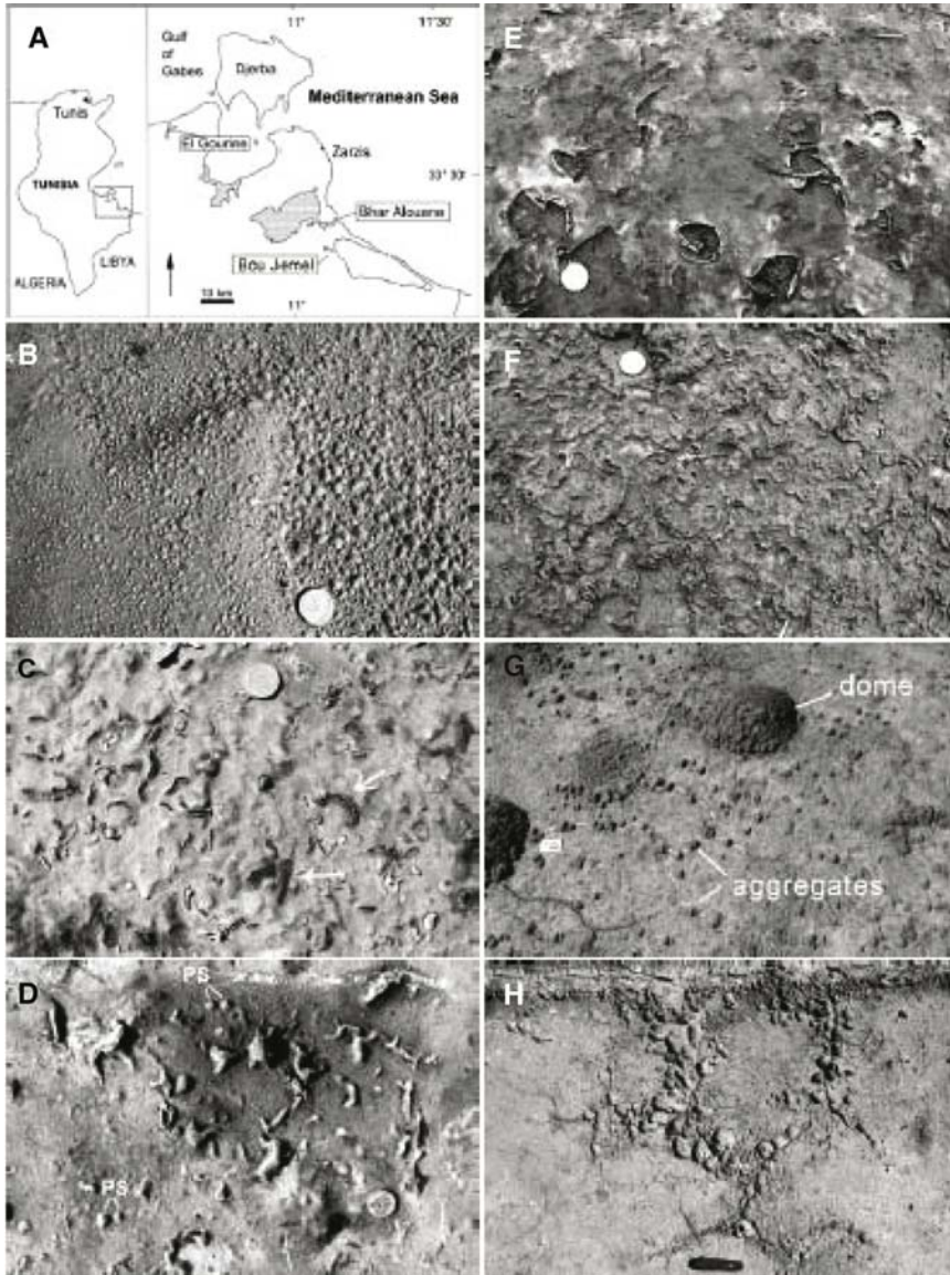
Figure 8. Location and structures related to mats developed in Tunisian supratidal zones and sabkhas. (A) Location of study sites Bhar A louane (B–D), El Gourine (E, F), and Bou Jemel sabkha (G, H). Scale (coin) is 24 mm in B–F. (B) Photosynthetic domes (PS-domes) trapped below EPS film in thin mat of coccoidal cyanobacteria. (C) Small sigmoidal to curved shrinkage cracks. Arrows indicate cracks with microbial activity triggered by uprisings of groundwater. (D) Several generations of overgrown shrinkage cracks and PS-domes (PS). (E) Subcircular crack openings with curled margins in thin mat layer. (F) Several generations of overgrown circular cracks. (G) Aggregates and domes of coccoid cyanobacteria and gypsum crystals, related to desiccation cracks. (H) Domes of filamentous and coccoid cyanobacteria arranged along desiccation cracks. Scale is 8 cm.
