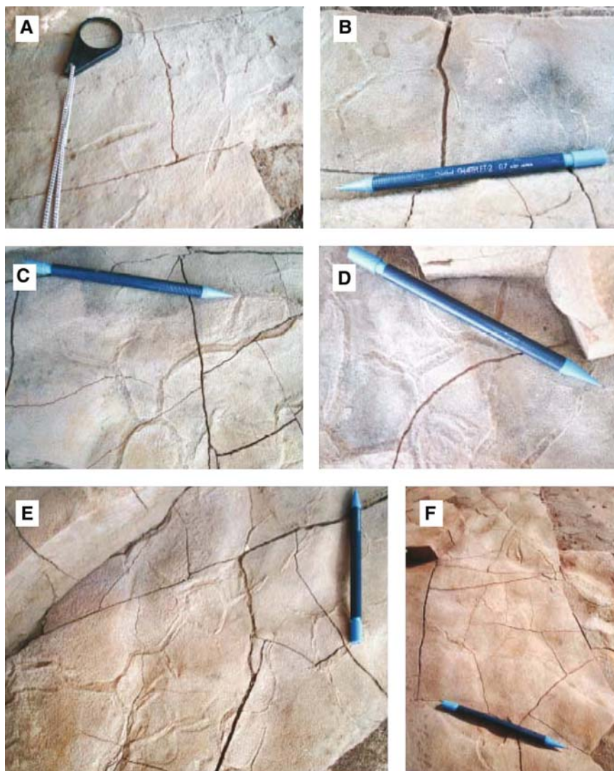
Figure 4. A variety of sand crack types observed within sandstone beds of the Makgabeng Formation. (A) Short, isolated, spindle-shaped cracks (hand lens for scale). (B) Apparent joining up of spindle-shaped cracks to form triradiate (“triple junction”) crack patterns (pen for scale). (C) Longer and more sinuous sand crack patterns, to which shorter, triradiate cracks appear to be joined – note the triradiate crack at the pen-tip, which appears to be a separate crack system, adjacent to rather than connected to the longer, curved features. (D) Triradiate crack set, between modern crack in sandstone bed and middle of pen (scale), which appears to be incompletely linked to sinuous, longer crack features. (E) As longer cracks develop, they become even more sinuous, even developing circular patterns (pen for scale). (F) Larger-scale view of rippled upper sandstone bed surface in the Makgabeng Formation, covered by a variety of sand cracks, mainly of higher sinuosity and circular geometry.
