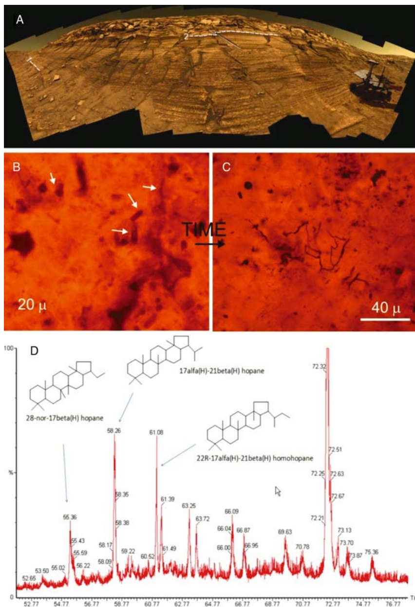
Figure 4. Burns Formation at the Burns Cliff in the Endurance Crater of Meridiani (A), Pan cam image PIA03241 resulted of a false color composite mosaic (courtesy of NASA/JPL-Caltech). Whattanga and Wellington sedimentary boundaries (Grotzinger et al., 2005), showed as 1 and 2, respectively; grained-sulfates and the hematites in concretionary structures (blueberries). Both mineralogies have been identified as mineralogies giving some clues concerning to the acidic conditions of
